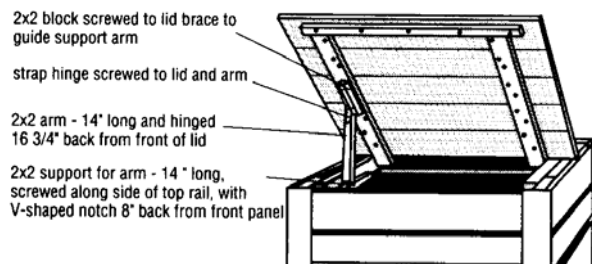
Figure 9 - Lid support detail.
